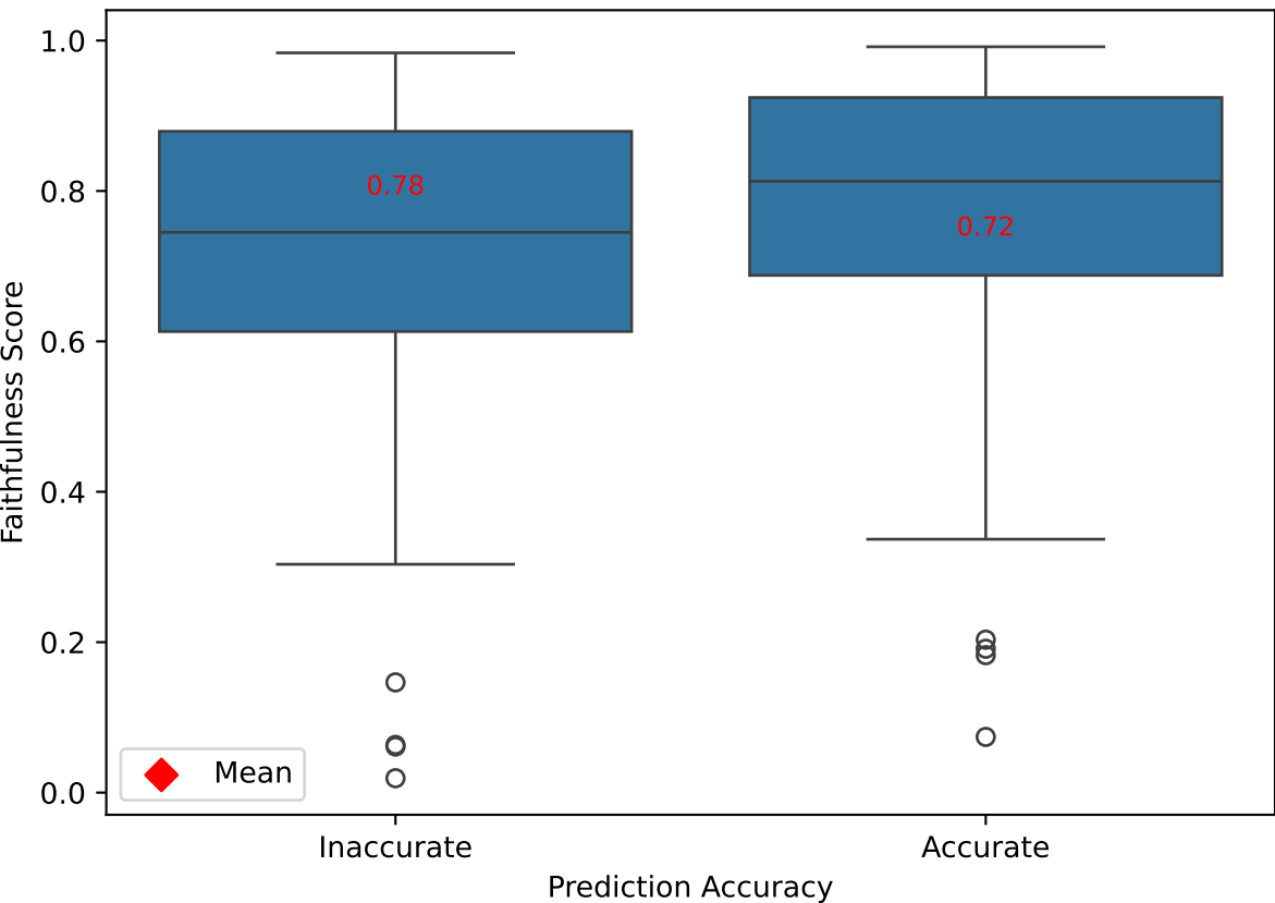
Faithfulness Score vs. Label Accuracy for UniEval
