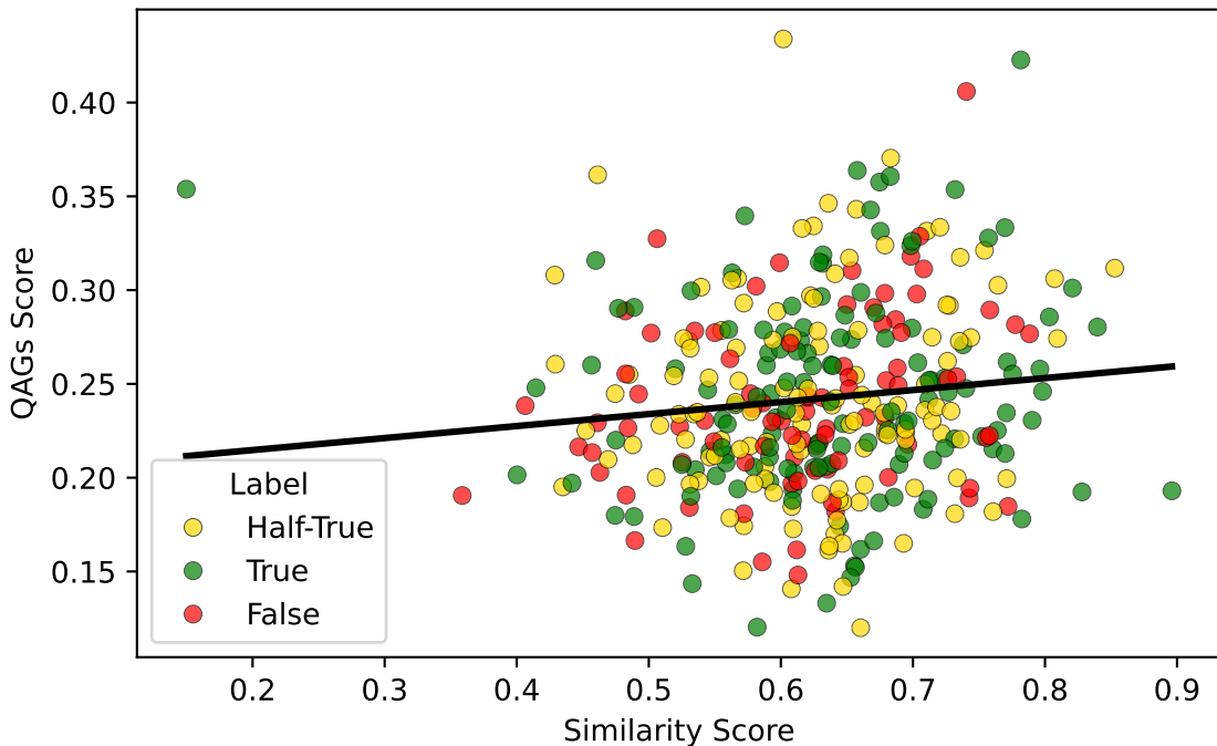
QAGs vs. Similarity (Spearman \rho = 0.14 )
