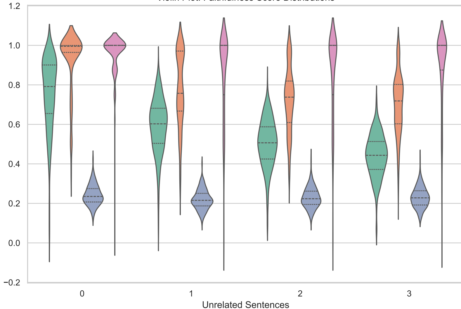
Violin Plot: Faithfulness Score Distributions
