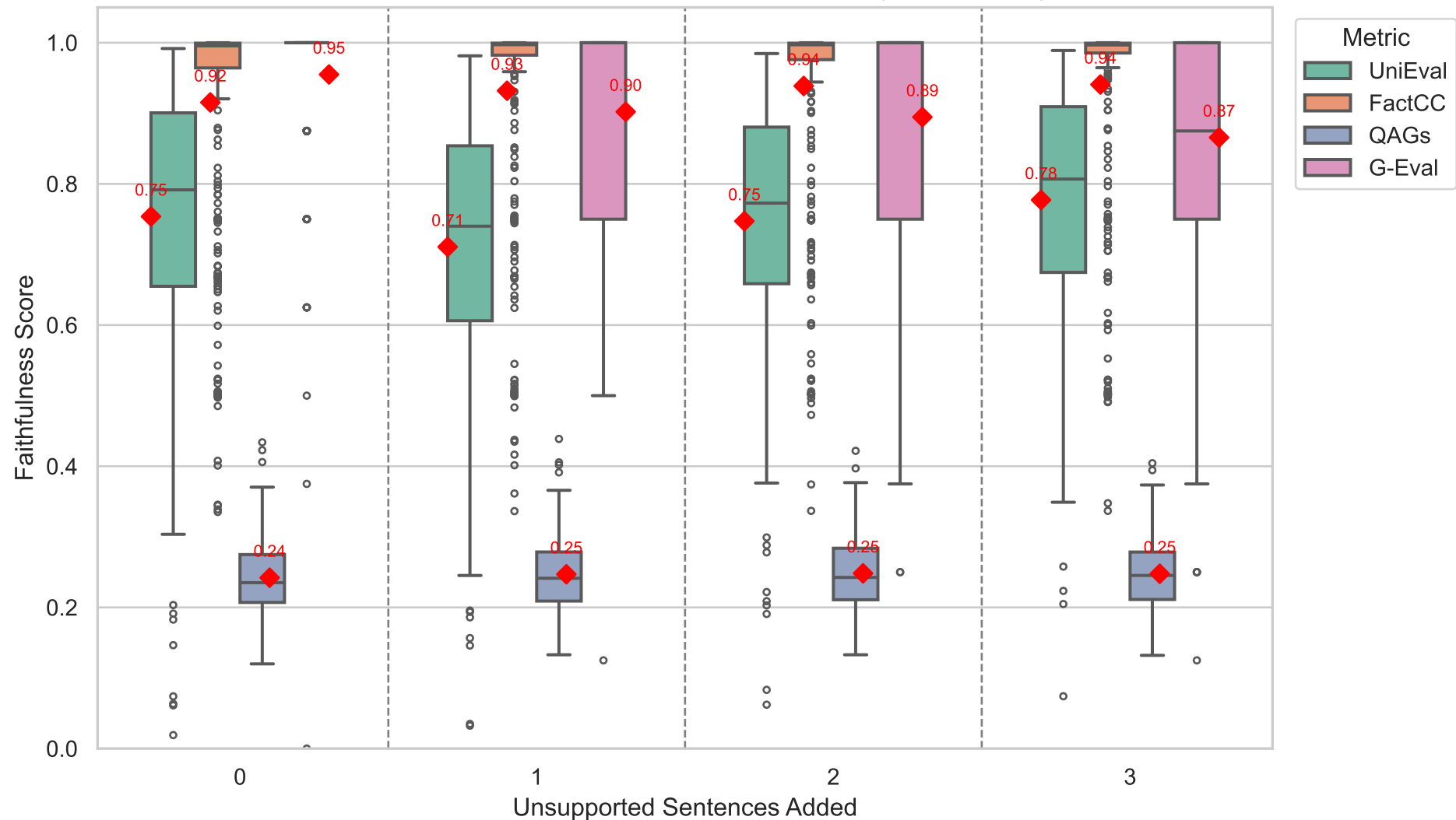
Box Plot: Faithfulness vs Unsupported Sentences (Means in Red)
