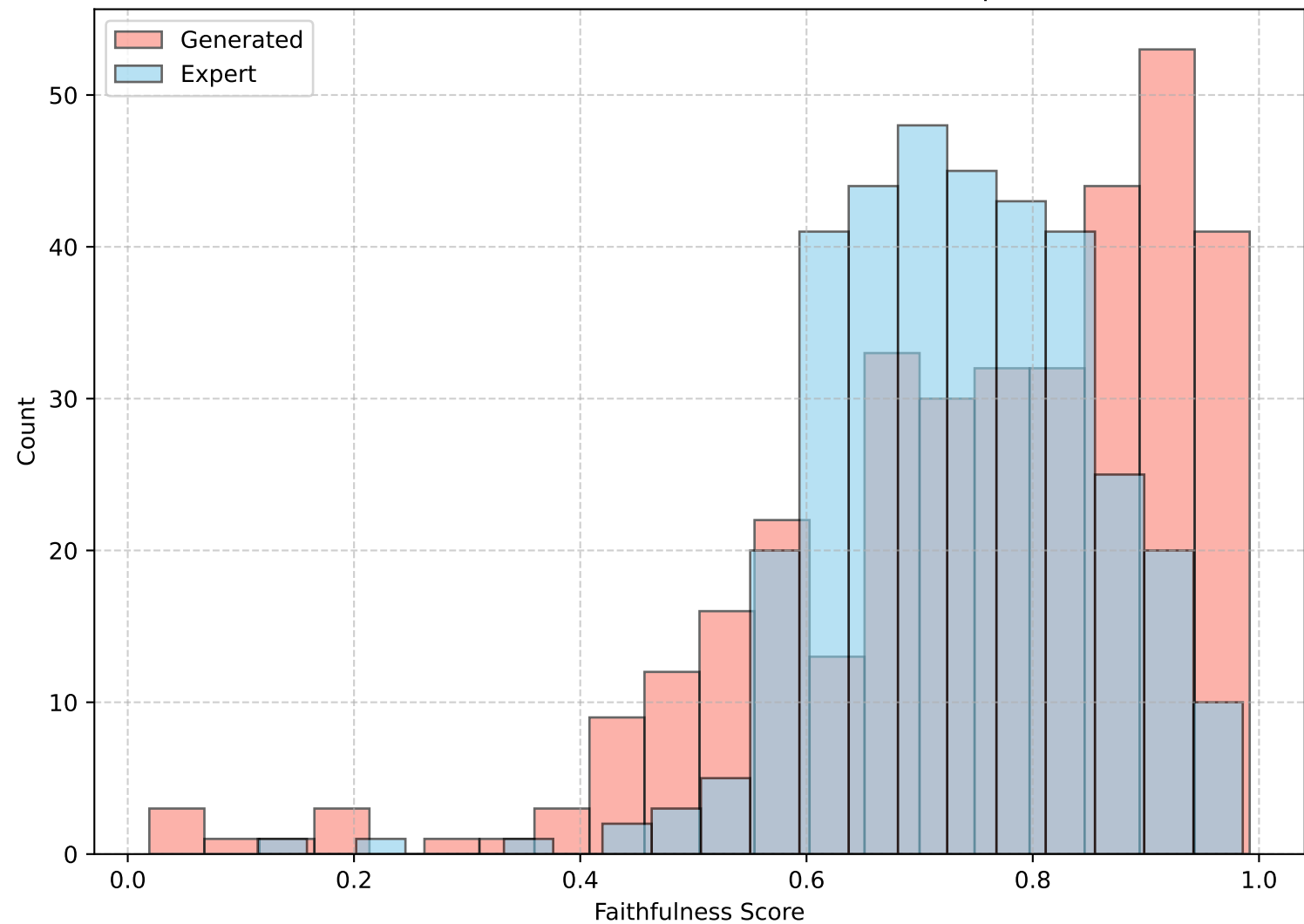
UniEval: Score Distribution (Generated vs. Expert)
