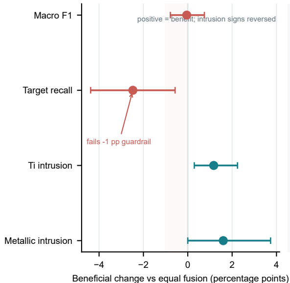
b Classification trade-off
