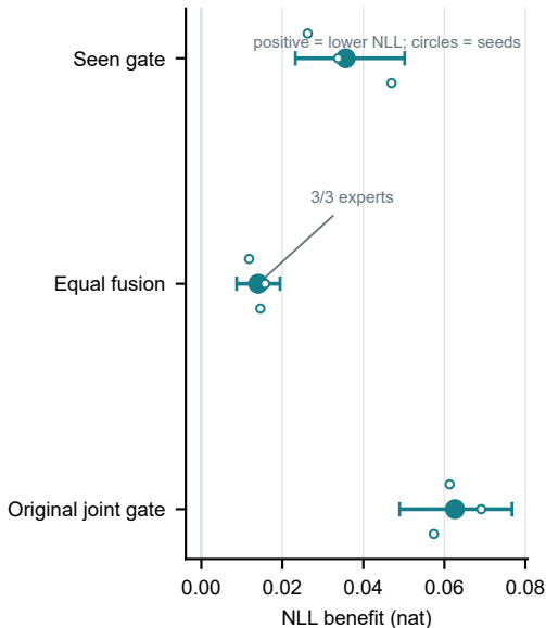
a Proper-scoring risk
