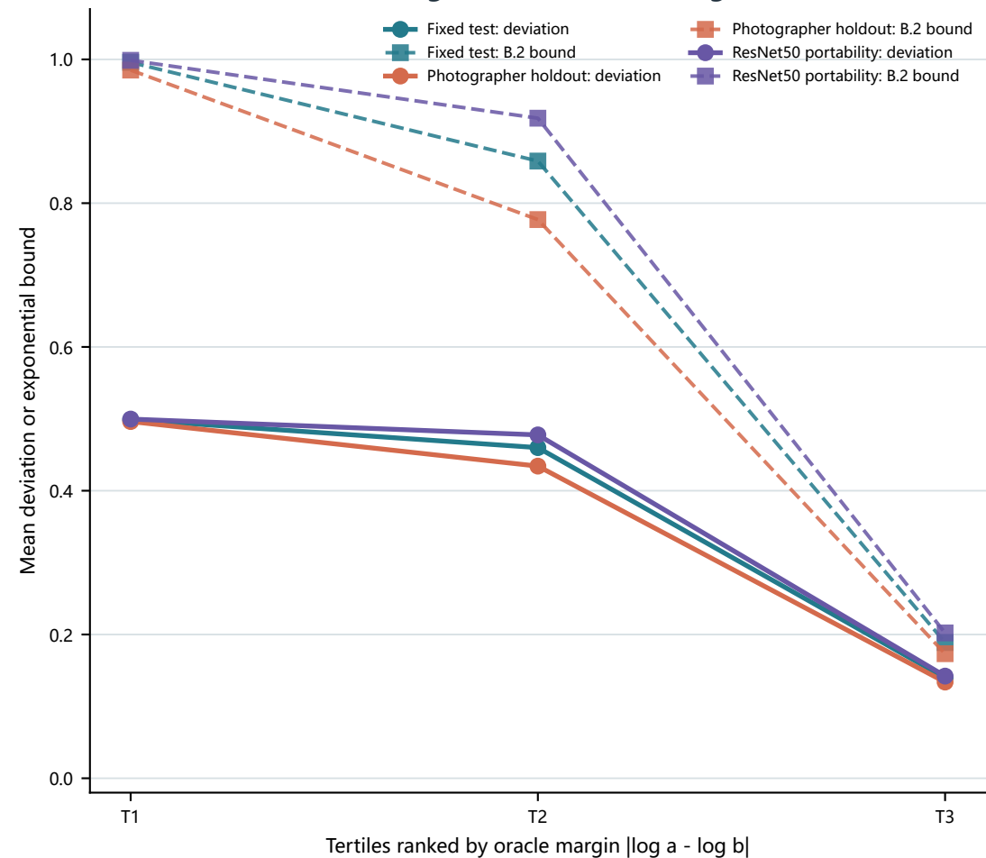
Theorem B.2: margin-stratified soft-target deviation
