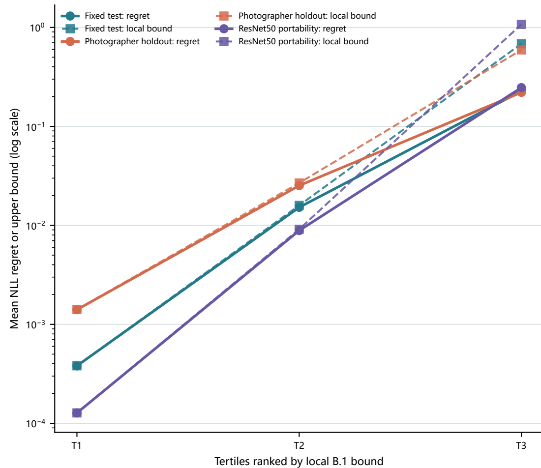
Theorem B.1: local B.1 bound strata
