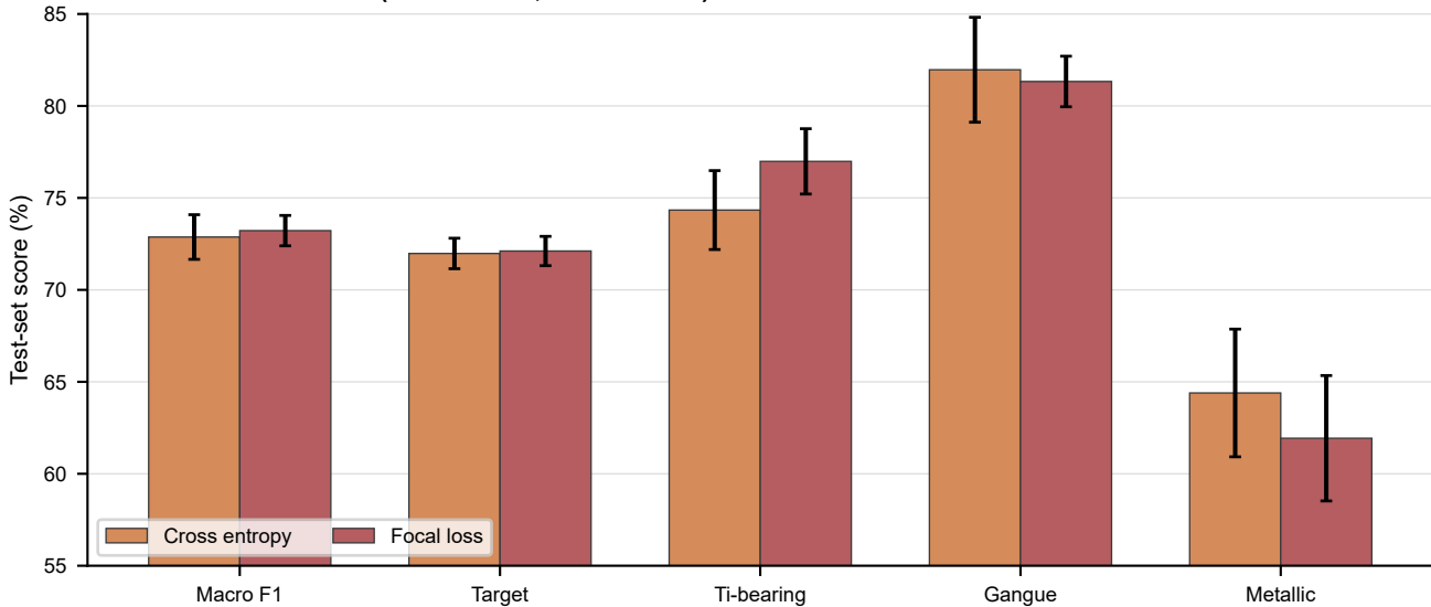
Loss-function ablation (three seeds, mean \pm SD)
