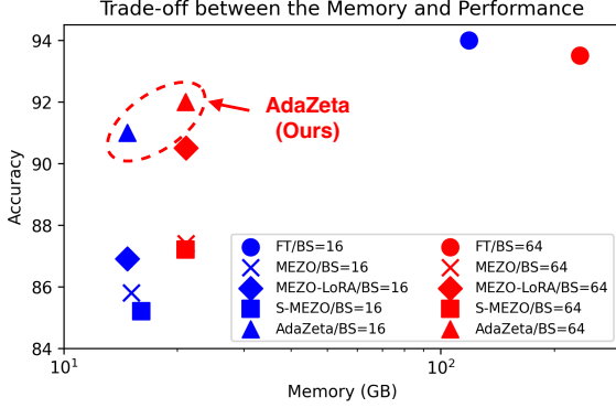
Figure 3: Trade-off between the accuracy and memory cost for different fine-tuning methods. We can observe that the AdaZeta method achieves the best accuracy among the memory-efficient methods.
