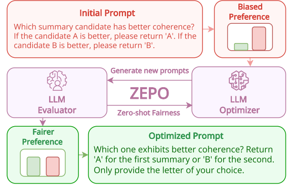
Figure 1: Illustration of the ZEPO pipeline. Given a manual prompt, the distribution of LLM preferences can be biased towards a certain class. ZEPO optimizes the prompt on a zero-shot fairness learning objective until the balance is achieved in the distribution.
