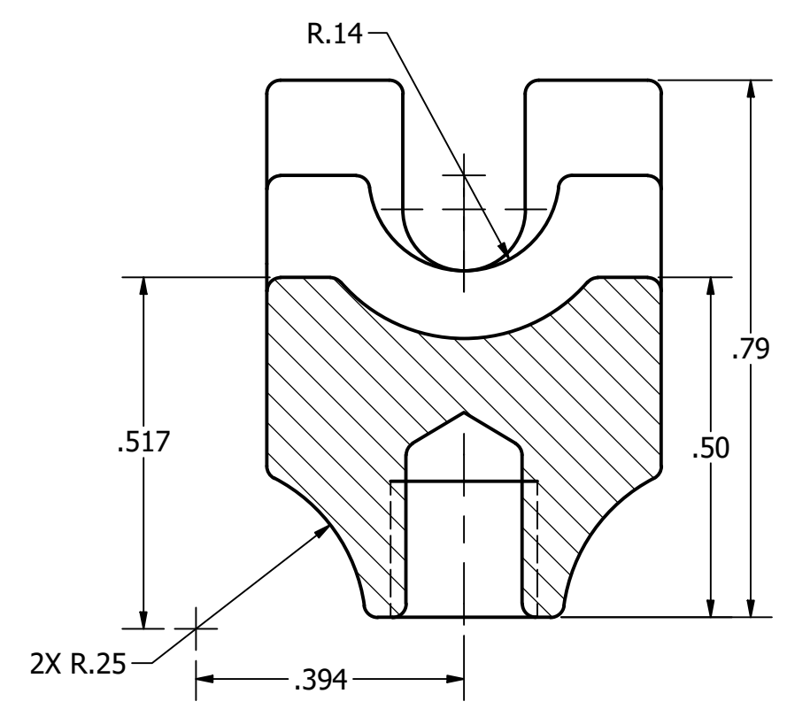
SECTION C-C
