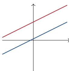
no solution
