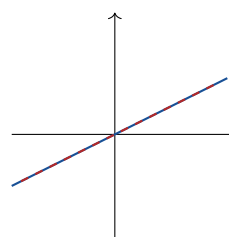
infinitely many
