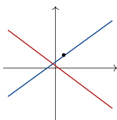
unique solution
