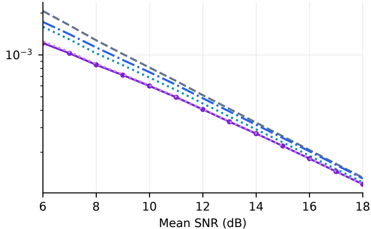
Fixed-coefficient basis-field MSE
