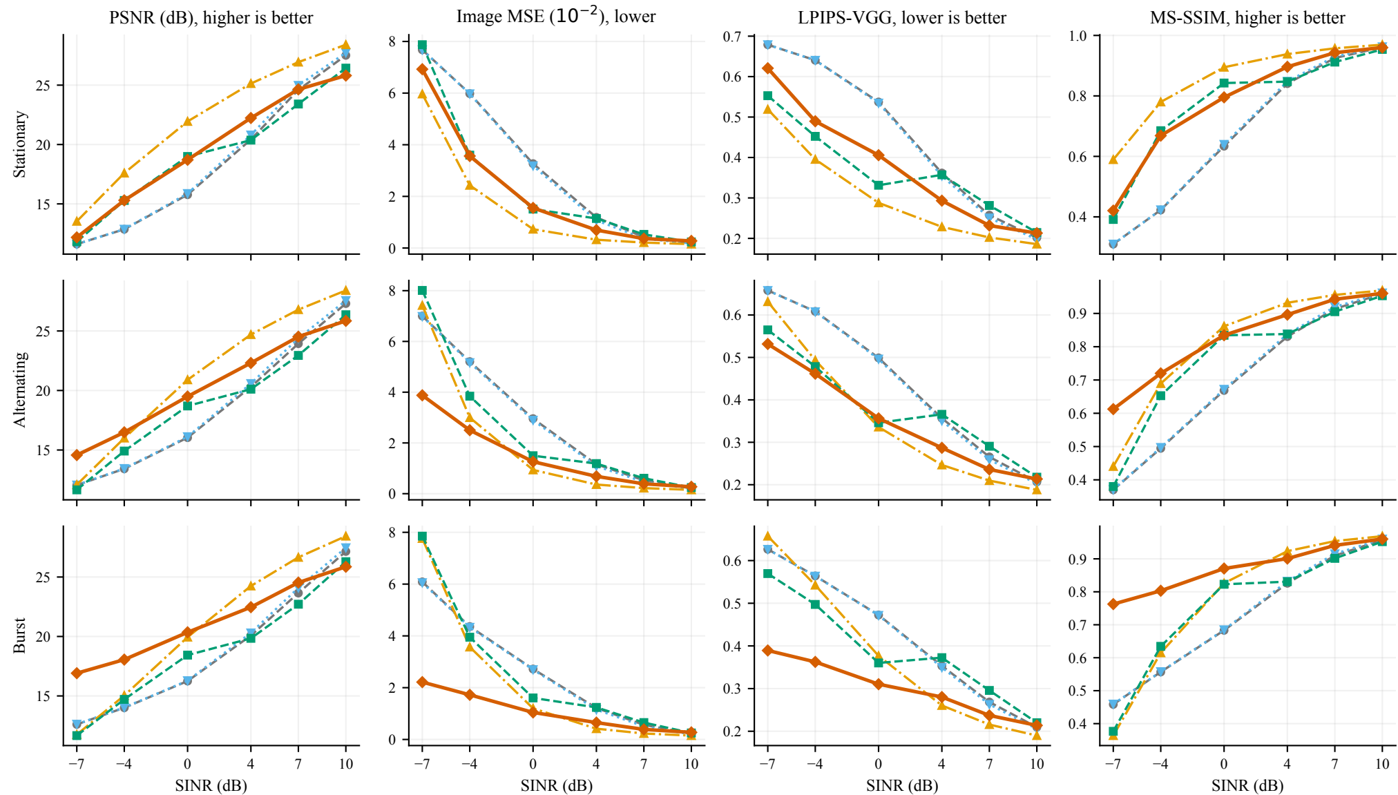
Exploratory paired validation. CDDM-RX: shared-prior, frozen-decoder port; oracle: true global SINR.
