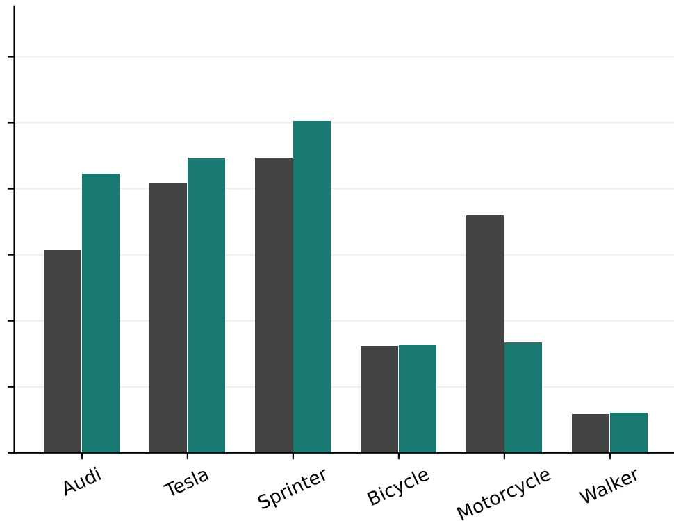
Mode hypotheses
