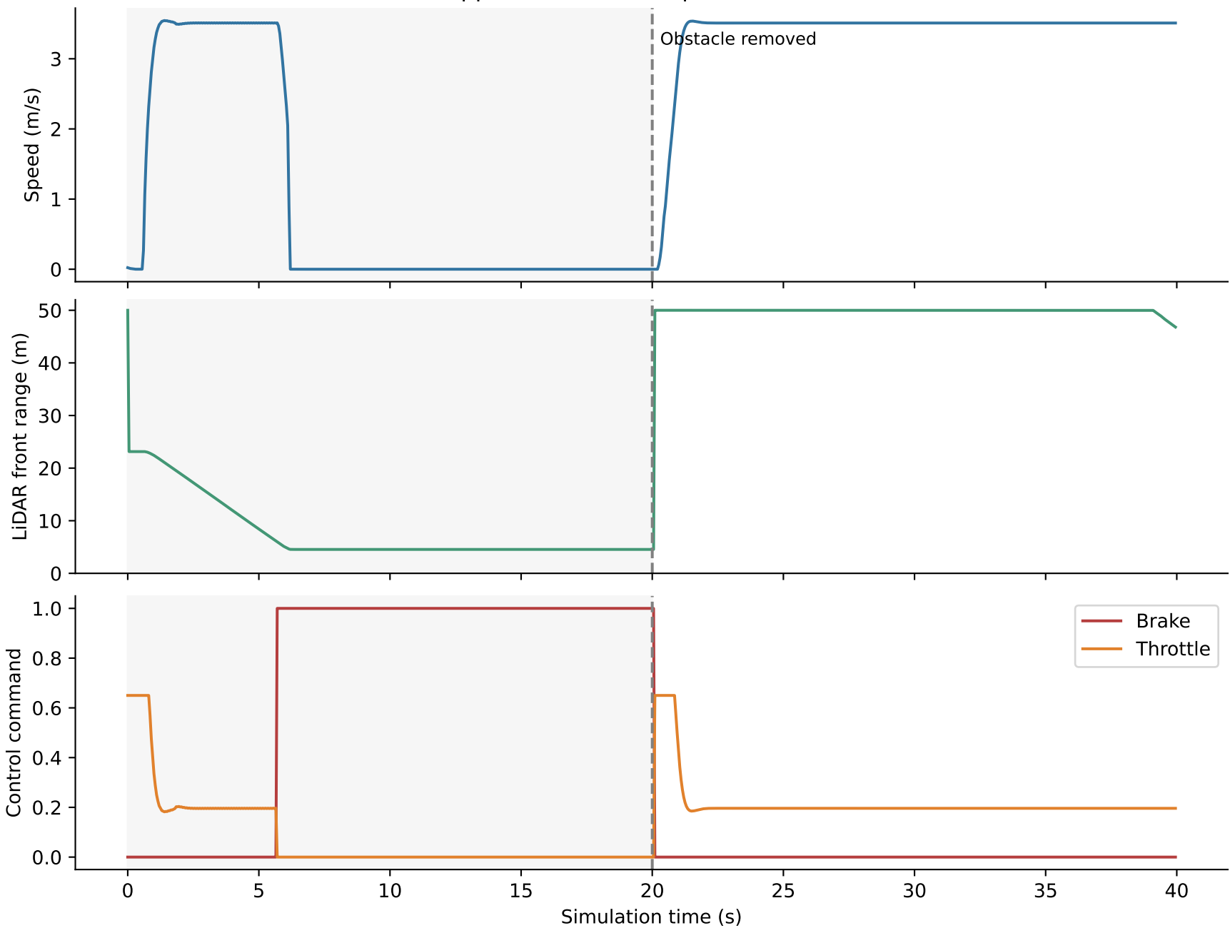
Sensor feedback: approach, brake, stop, resume after obstacle removal
