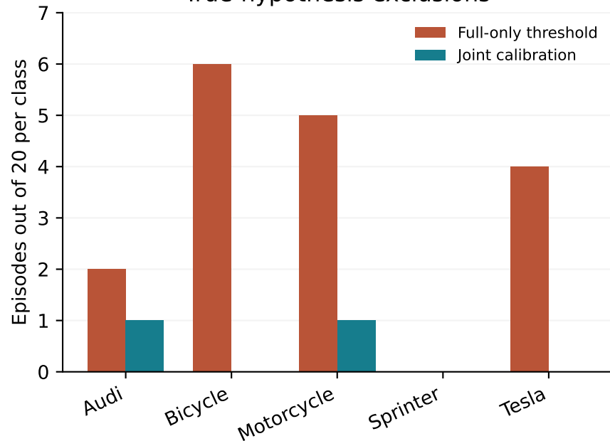
True-hypothesis exclusions
