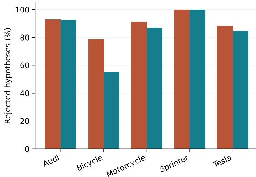
Translated-hypothesis diagnostic
