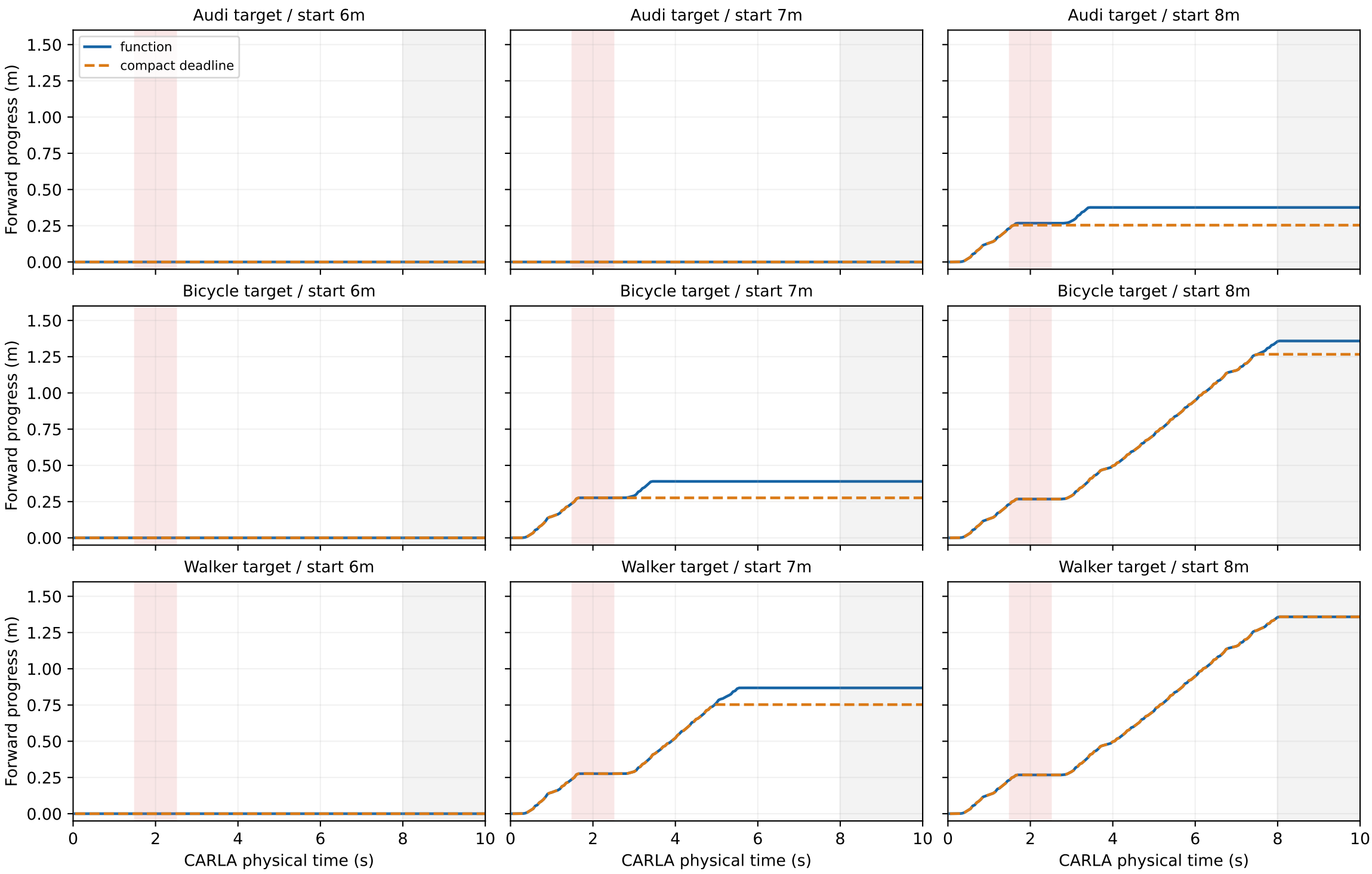
Near-hazard finite physical loop / 20ms modeled propagation Red: source packet dropout; gray: final full brake; no policy risk qualification
