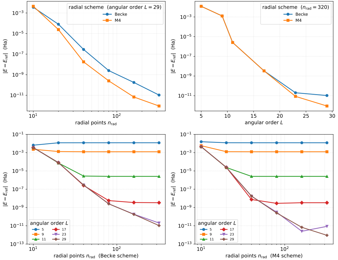
Figure 8: Two-dimensional (radial \times angular) grid convergence of the \text{H}_2^+ core-Hamiltonian ground-state (lowest-MO) energy, comparing the Becke and Treutler-Ahlrichs (M4) radial schemes on a shared Lebedev angular grid. Molecule: \text{H}_2^+ with protons at x = 0 and x = 1 bohr; basis: QZ4P. Top left: radial convergence at the finest angular order in the sweep ( L = 29 ). Top right: angular convergence at the finest radial grid ( n_{\text{rad}} = 320 ). Bottom: for each scheme, |E - E_{\text{ref}}| versus n_{\text{rad}} with one curve per angular order L \in \{5, 9, 11, 17, 23, 29\} , illustrating that each radial curve plateaus at a floor set by the angular order (and vice versa). The reference is the mean of the two schemes on the finest grid ( n_{\text{rad}} = 640 , L = 41 ), E_{\text{ref}} = -1.45175161440473 Ha (shared self-reference; the two schemes agree there to 7 \times 10^{-13} Ha). The ordinate is |E - E_{\text{ref}}| .
