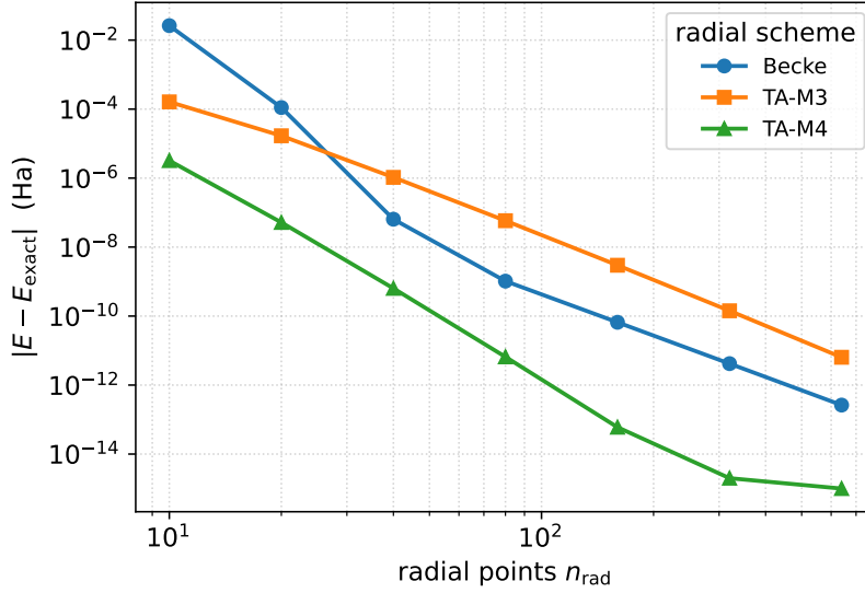
Figure 6: We compute the lowest-MO energy of a single hydrogen atom for three radial quadrature schemes: Becke, Treutler-Ahlrichs (M3) ( \alpha = 0 ) and (M4) ( \alpha = 0.6 ), both with element scaling \xi(\text{H}) = 0.8 . As our basis set we chose QZ4P (ADF Slater-type). The angular grid is a Lebedev grid fixed at order L = 29 . The radial point count is swept over n_{\text{rad}} \in \{10, 20, 40, 80, 160, 320, 640\} . The reference is the exact non-relativistic 1s energy of the hydrogen atom, E_{\text{exact}} = -0.5 Ha, so the ordinate |E - E_{\text{exact}}| is pure quadrature error.
