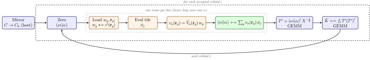
Figure 4: Control-flow of the neighbor-tiled RI-K kernel ( compute_exact_exchange_tiled ). The occupied orbitals are treated one at a time: orbital i is folded into the quadrature weights via c^i(\mathbf{r}_g) = \sum_k C_{ki} \phi_k(\mathbf{r}_g) , the three-center integral (\nu i | \alpha) is built by the tiled team kernel (each neighbor tile of \phi_j evaluated once and reused across all auxiliary functions \alpha ), and \tilde{K}_{\mu\nu} is accumulated by two host GEMMs applying X^{-\frac{1}{2}} . Colors as in Figure 3.
