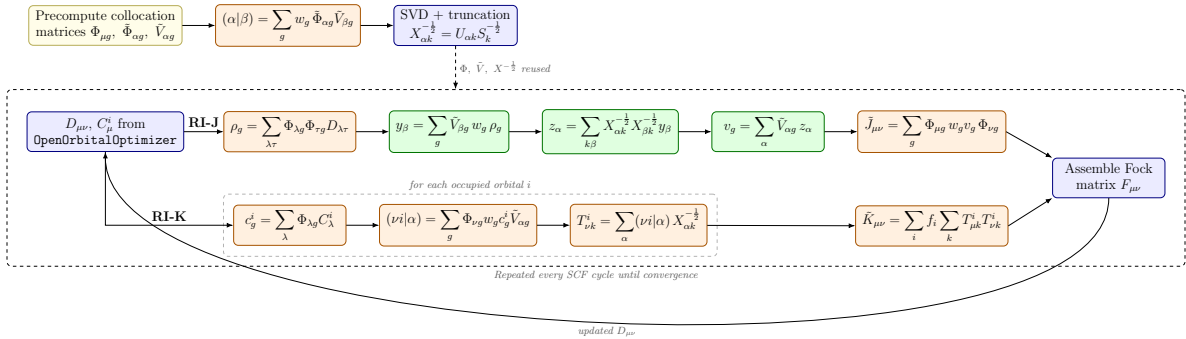
Figure 2: Control-flow of the dense RI-J and RI-K integral routines, annotated with the underlying equations. The boxes in the top row form the one-time startup phase; everything inside the outer dashed region is re-evaluated in every SCF cycle. Boxes are colored by operation type: blue for host orchestration and interaction with the external SCF library, yellow for pre-computed data held in device memory, orange for dense matrix-matrix products (GEMM), and green for matrix-vector products (GEMV) and element-wise scaling. The inner dashed box marks the loop over occupied orbitals in the RI-K scheme. The Fock/Kohn-Sham assembly is drawn schematically.
