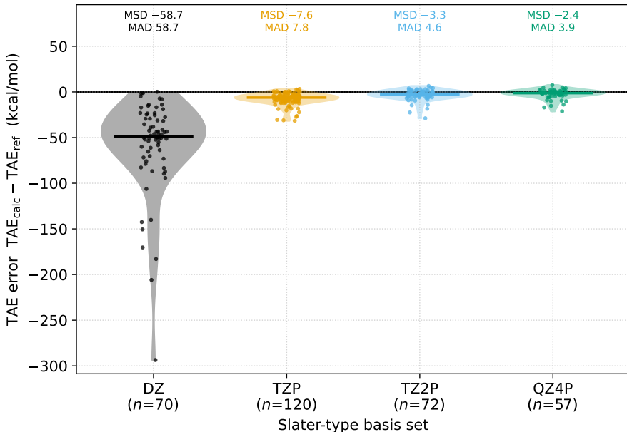
Figure 11: Distribution of the signed error in the W4-11 total atomization energies, one violin per Slater-type basis set, with the number of converged reactions given below each label. Method is unrestricted B3LYP (Libxc 56 hyb_gga_xc_b3lyp3 , the VWN3 parametrization) with the dense algorithm. The grid is TA-M4 radial with n_{\text{rad}} = 100 and Lebedev order L = 35 with robust pruning and uniform radial sizing. The linear dependence threshold of 10^{-4} is applied uniformly to all four basis sets. Reference values are the zero-point exclusive, non-relativistic, clamped-nuclei atomization energies of Ref. 18 Individual reactions are overlaid as jittered points and the horizontal bar marks the median. The summary statistics are given in Table 6.
