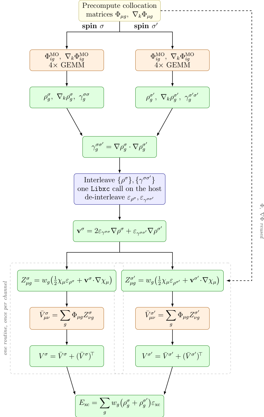
Figure 3: Control-flow of the spin-unrestricted GGA routine compute_gga_1sda , annotated with the underlying equations. The two spin channels run as parallel columns and join twice: once to form the cross invariant \gamma^{\sigma\sigma'} , which is the only quantity that couples them, and once at the end for the energy. Boxes are colored by operation type: blue for host-side orchestration and the functional evaluation, which has to run on the CPU; yellow for pre-computed data held in device memory; orange for dense matrix-matrix products (GEMM); and green for team-parallel kernels over the quadrature grid. The two dashed regions mark the per-channel assembly, which is a single routine invoked once per spin with its own \varepsilon_{\rho^\sigma} and \mathbf{v}^\sigma : only the construction of \mathbf{v}^\sigma above it is specific to the unrestricted case.
