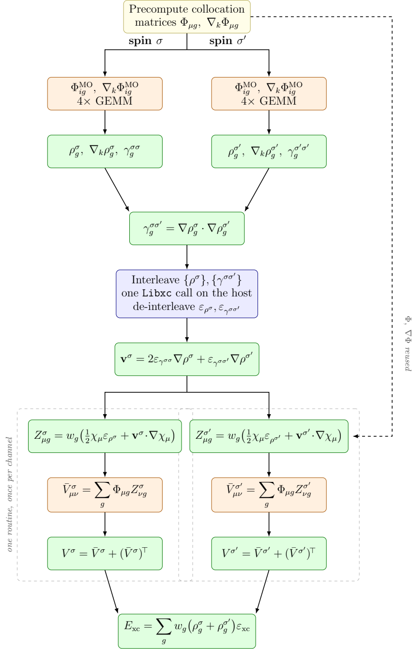
Figure 3: Control-flow of the spin-unrestricted GGA routine compute_gga_1sda , annotated with the underlying equations. The two spin channels run as parallel columns: once to form the cross invariant \gamma^{\sigma\sigma'} , which is the only quantity that couples them, and once at the end for the energy. Boxes are colored by operation type: blue for host-side orchestration and the functional evaluation, which has to run on the CPU; yellow for pre-computed data held in device memory; orange for dense matrix–matrix products (GEMM); and green for team-parallel kernels over the quadrature grid. The two dashed regions mark the per-channel assembly, which is a single routine invoked once per spin with its own \varepsilon_{\rho^\sigma} and \mathbf{v}^\sigma : only the construction of \mathbf{v}^\sigma above it is specific to the unrestricted case.
