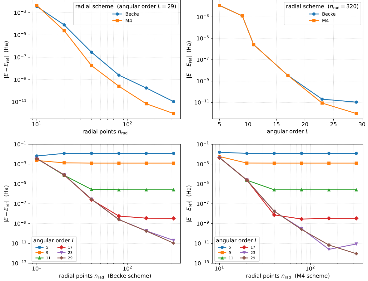
Figure 8: Two-dimensional (radial \times angular) grid convergence of the H_2^+ core-Hamiltonian ground-state (lowest-MO) energy, comparing the Becke and Treutler-Ahlrichs (M4) radial schemes on a shared Lebedev angular grid. Molecule: H_2^+ with protons at x = 0 and x = 1 bohr; basis: QZ4P. Top left: radial convergence at the finest angular order in the sweep ( L = 29 ). Top right: angular convergence at the finest radial grid ( n_{\text{rad}} = 320 ). Bottom: for each scheme, |E - E_{\text{ref}}| versus n_{\text{rad}} with one curve per angular order L \in \{5, 9, 11, 17, 23, 29\} , illustrating that each radial curve plateaus at a floor set by the angular order (and vice versa). The reference is the mean of the two schemes on the finest grid ( n_{\text{rad}} = 640 , L = 41 ), E_{\text{ref}} = -1.45175161440473 Ha (shared self-reference; the two schemes agree there to 7 \times 10^{-13} Ha). The ordinate is |E - E_{\text{ref}}| .
