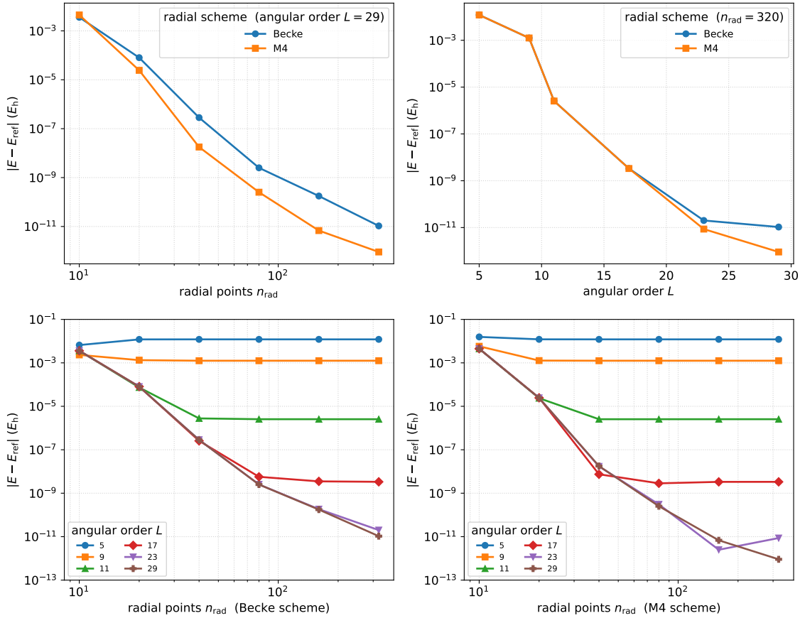
Figure 8: Two-dimensional (radial \times angular) grid convergence of the \text{H}_2^+ core-Hamiltonian ground-state (lowest-MO) energy, comparing the Becke and Treutler–Ahlich (M4) radial schemes on a shared Lebedev angular grid. Molecule: \text{H}_2^+ with protons at x = 0 and x = 1 bohr; basis: QZ4P. Top left: radial convergence at the finest angular order in the sweep ( L = 29 ). Top right: angular convergence at the finest radial grid ( n_{\text{rad}} = 320 ). Bottom: for each scheme, |E - E_{\text{ref}}| versus n_{\text{rad}} with one curve per angular order L \in \{5, 9, 11, 17, 23, 29\} , illustrating that each radial curve plateaus at a floor set by the angular order (and vice versa). The reference is the mean of the two schemes on the finest grid ( n_{\text{rad}} = 640 , L = 41 ), E_{\text{ref}} = -1.45175161440473 E_h (shared self-reference; the two schemes agree there to 7 \times 10^{-13} E_h ). The ordinate is |E - E_{\text{ref}}| .
