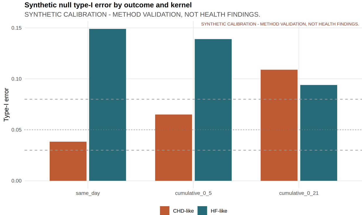
Figure 1: Methods feasibility only — synthetic M|D null Type I by outcome and kernel. Not a CHD/HF health result.
