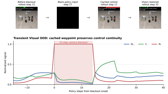
Fig. 5. Camera blackout on the Object suite. DUET holds the last reliable absolute waypoint while the image is invalid and resumes adaptive dual-action control when vision returns. The lower panel aggregates 500 episodes aligned to blackout onset.
