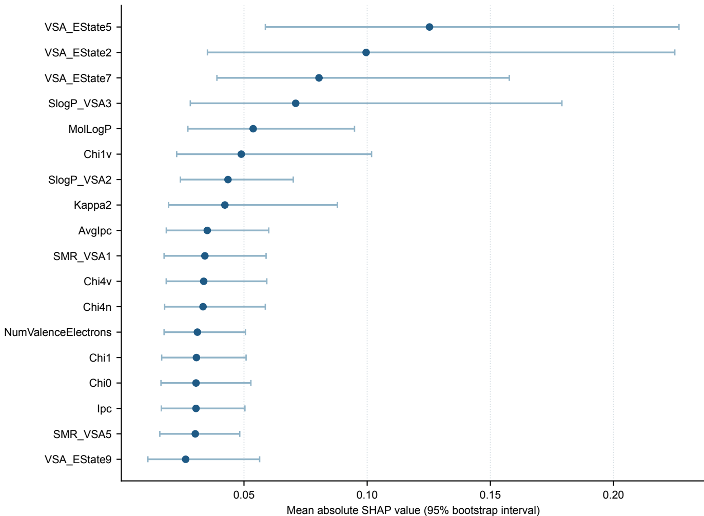
Bootstrap SHAP stability for 18 RDKit descriptors 500 refits; median Spearman \rho = 0.658 (95% interval 0.308–0.860)
