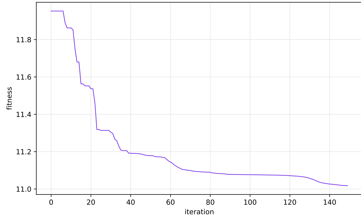
PSO Convergence (scaled fitness)
