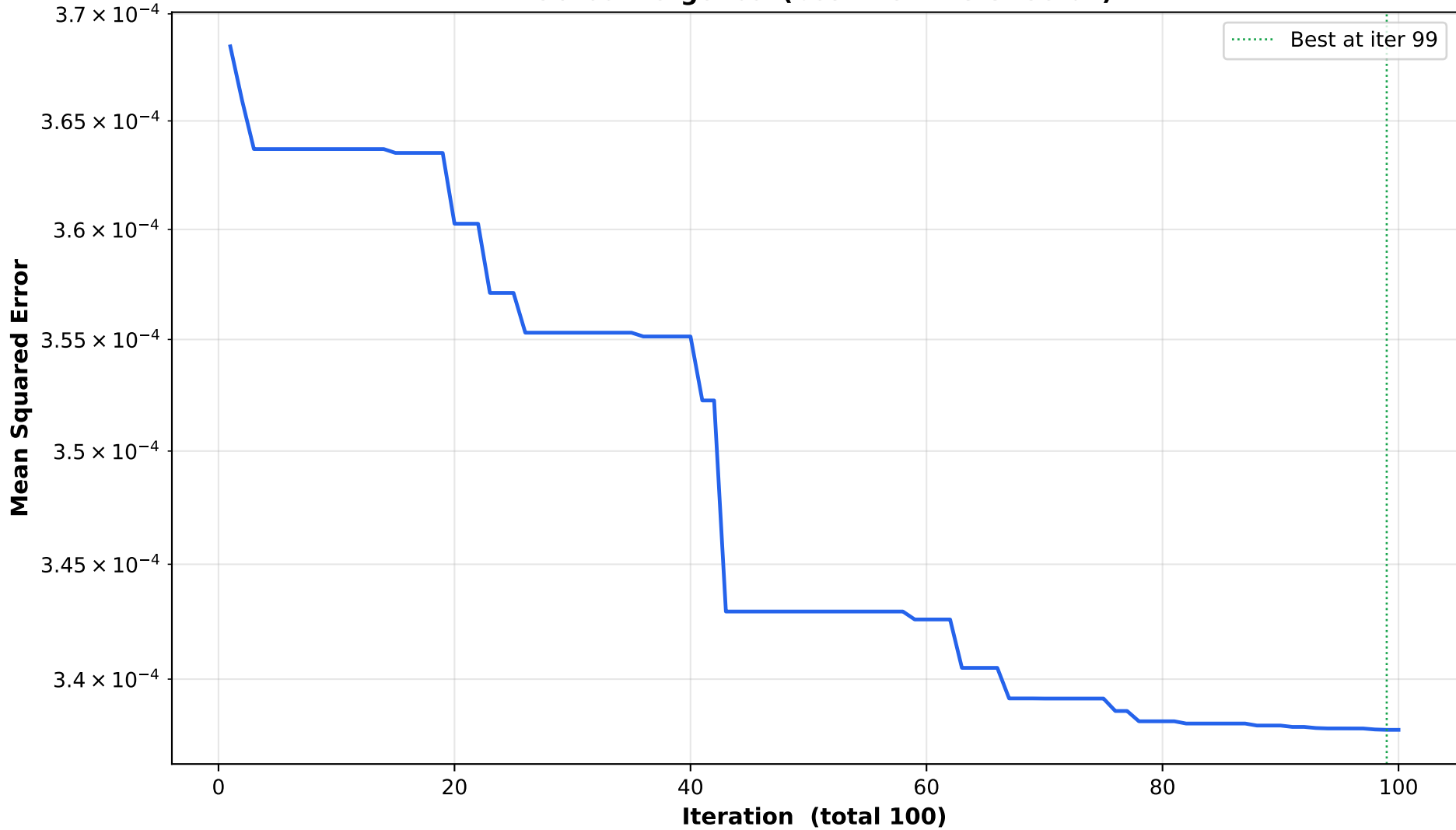
PSO Convergence (best MSE = 3.378e-04)
