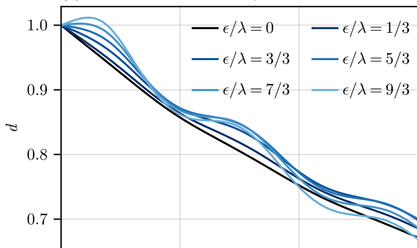
(a) Front vertical diffusivity
