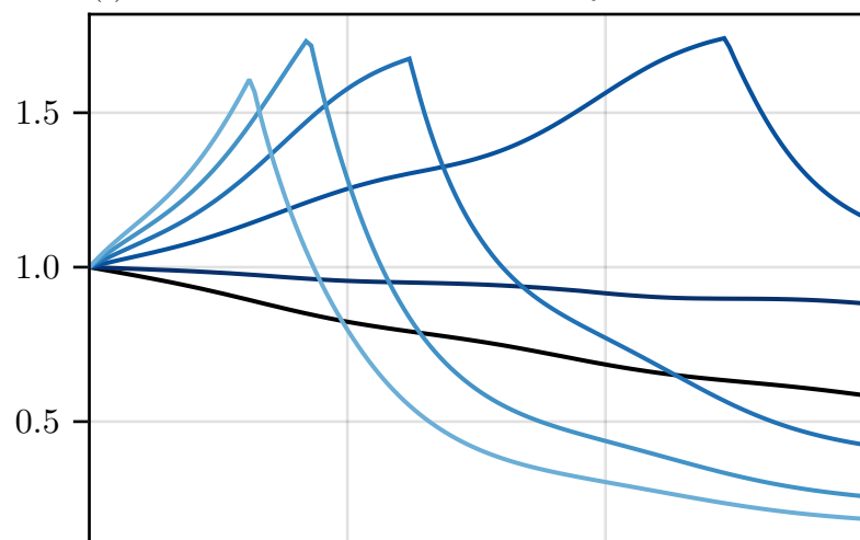
(f) Filament horizontal diffusivity
