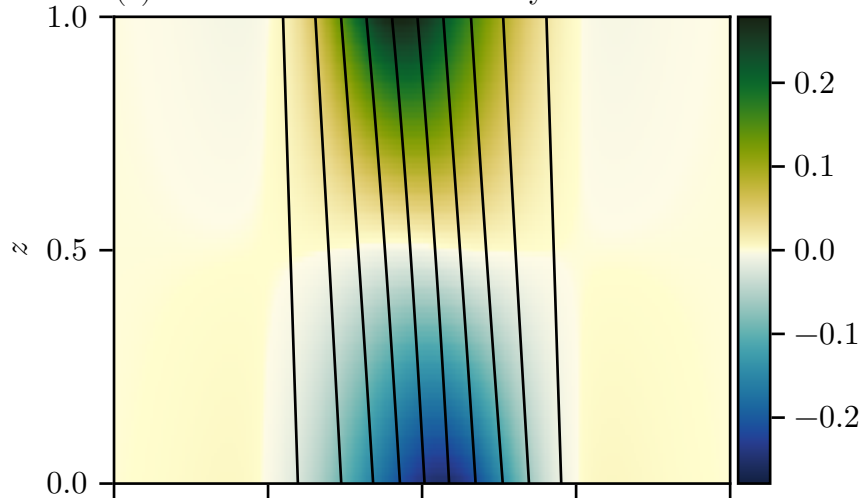
(g) Front horizontal viscosity
