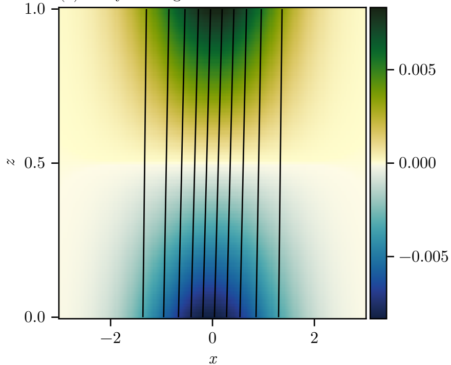
(a) Early frontogenesis v^0
