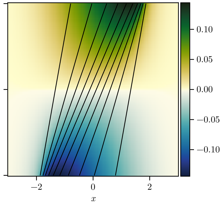
(b) Late frontogenesis v^0
