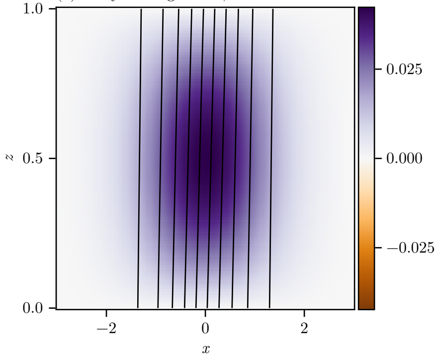
(a) Early frontogenesis \psi^0
