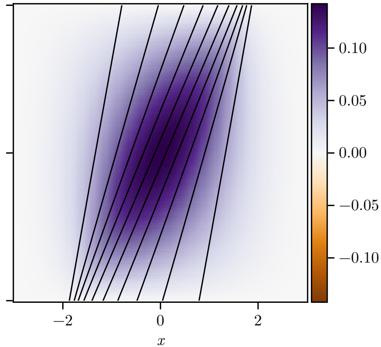
(b) Late frontogenesis \psi^0
