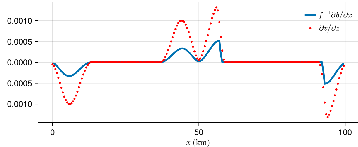
Thermal-wind balance, (y,z)=(75\text{km},60\text{m})
