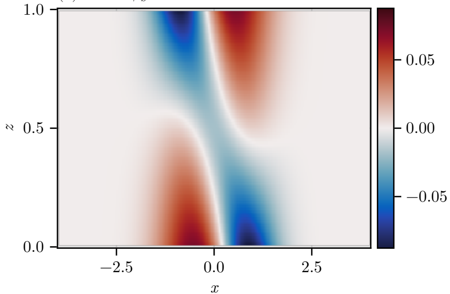
(a) Front \psi_s^1 error
