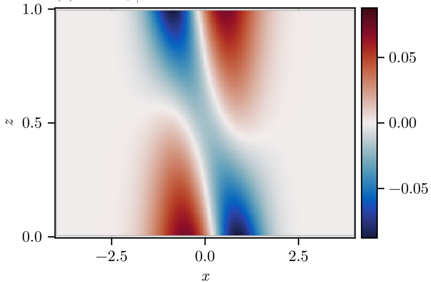
(a) Front \psi_\gamma^1 error
