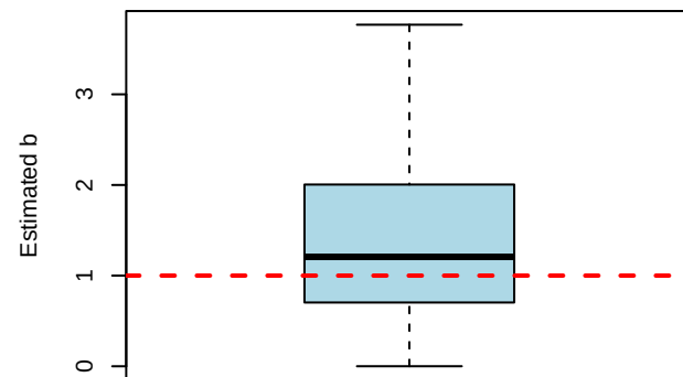
Scenario 3: b (True = 1)
