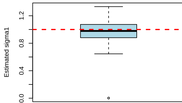
Scenario 2: sigma1 (True = 1)
