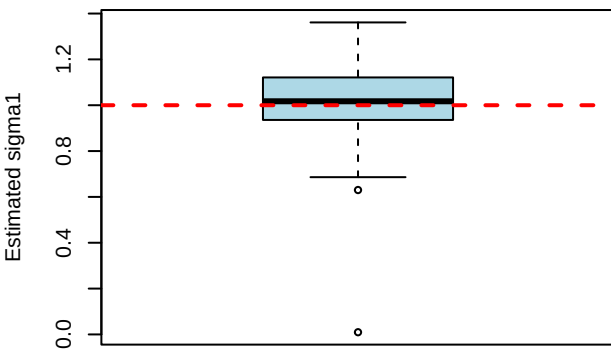
Scenario 1: sigma1 (True = 1)
