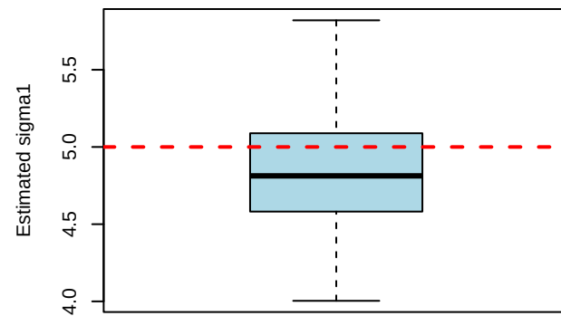
Scenario 3: sigma1 (True = 5)
