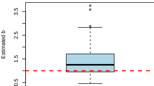
Scenario 1: b (True = 1)
