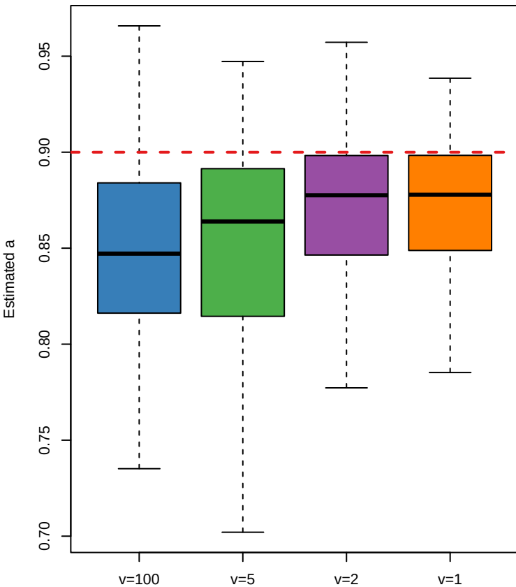
Estimated 'a' across Degrees of Freedom
