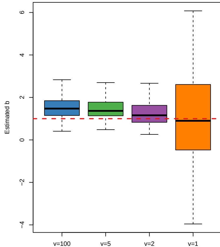
Estimated 'b' across Degrees of Freedom
