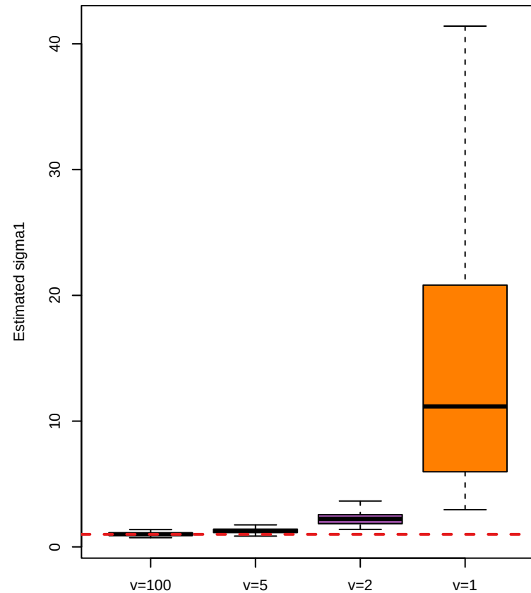
Estimated 'sigma1' across Degrees of Freedom
