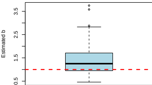
Scenario 1: b (True = 1)
