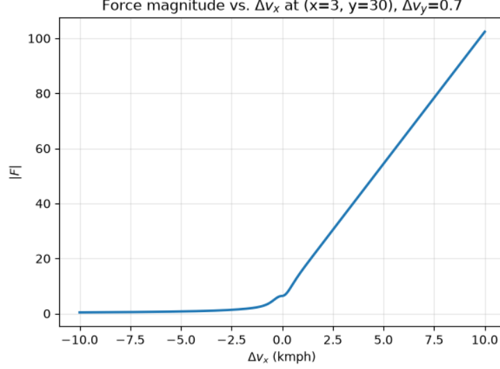
Figure 7: Force magnitude vs. \Delta v_x under Formulation 2.
