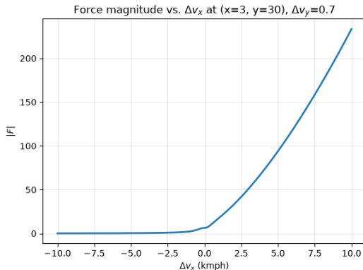
Force magnitude vs. \Delta v_x under Formulation 3
