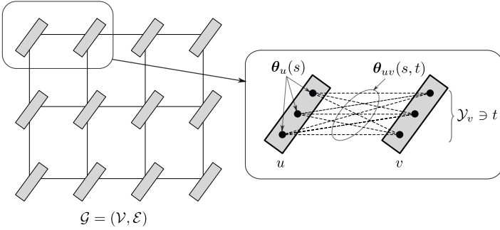
Figure 1.4: Example of a labeling problem with grid structure. On the left, graph nodes are denoted with inclined rectangles, lines connecting nodes correspond to graph edges. On the right, two neighboring nodes are shown. Black circles inside rectangles correspond to the labels s in the node u (left rectangle) and t in the node v (right rectangle). Dashed lines correspond to each label pair s, t with an assigned pairwise cost \theta_{uv}(s, t) .
