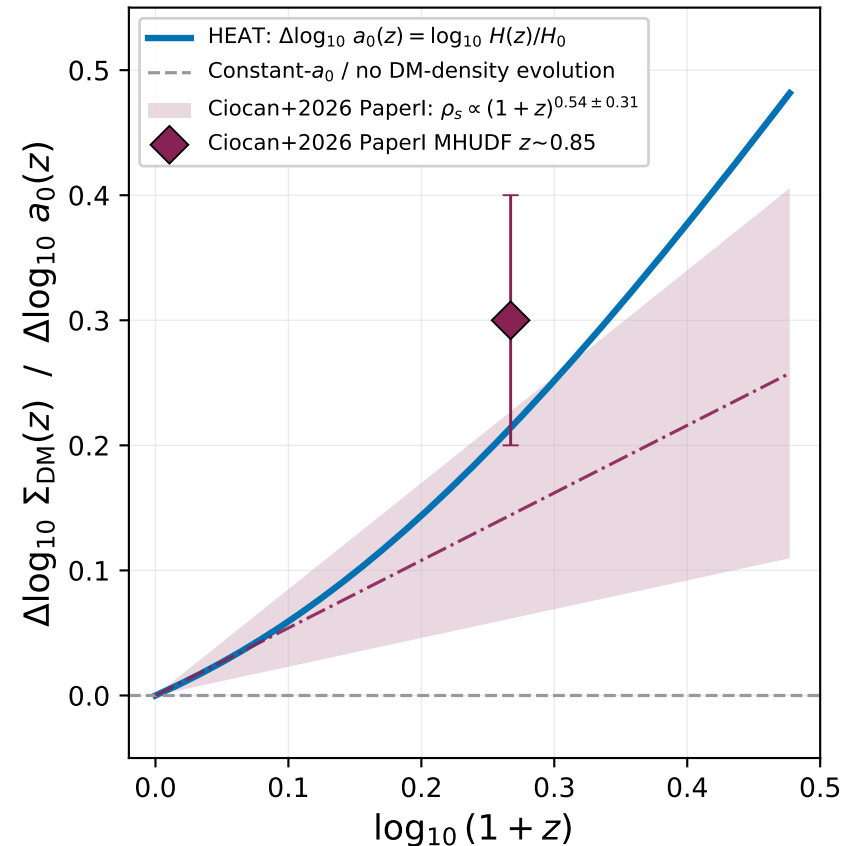
(b) Halo-density evolution: HEAT vs Paper I
