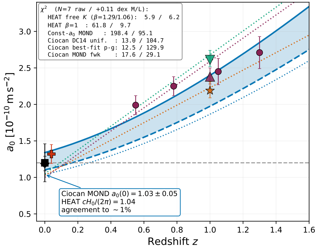
(a) a_0(z) : HEAT vs Ciocan+2026 (Paper III)
