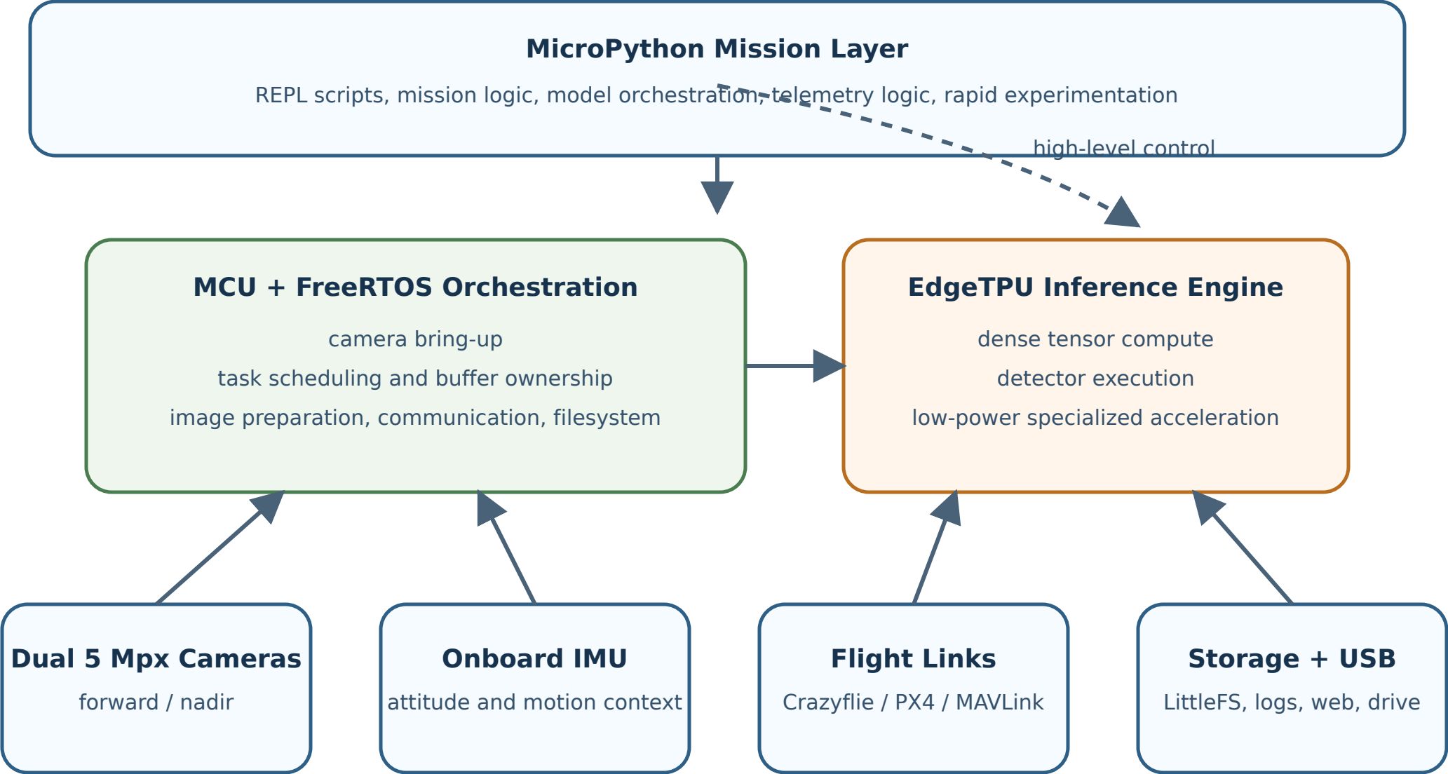
Layered view: sensing hardware - RTOS host orchestration - EdgeTPU inference - MicroPython experimentation surface
