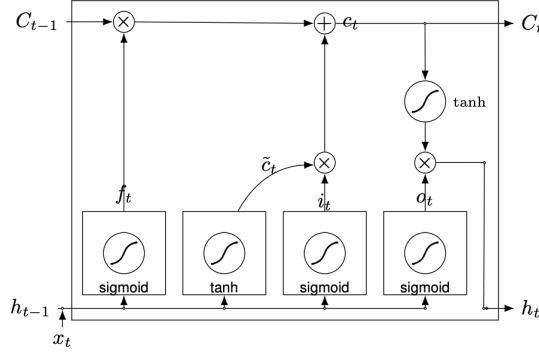
Figure 3: LSTM cell architecture [2]
