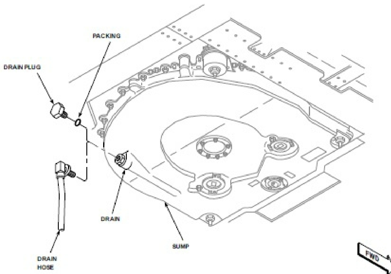
Figure 2. Drain Main Transmission.
