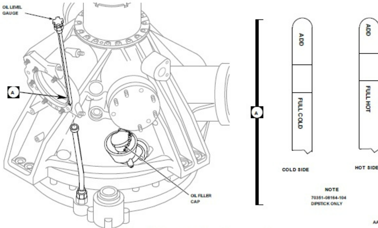
Figure 1. Service Main Transmission.
