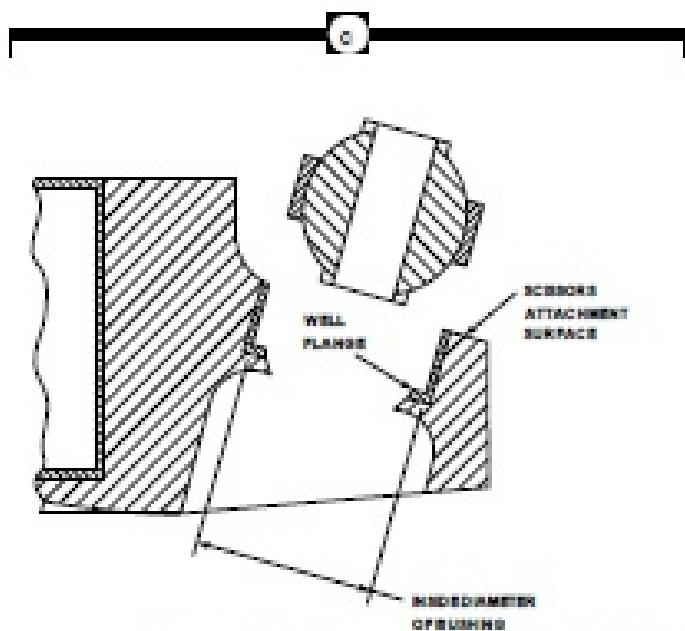
Figure 1. Replace Swashplate Scissors Attachment Spherical Bearing.
