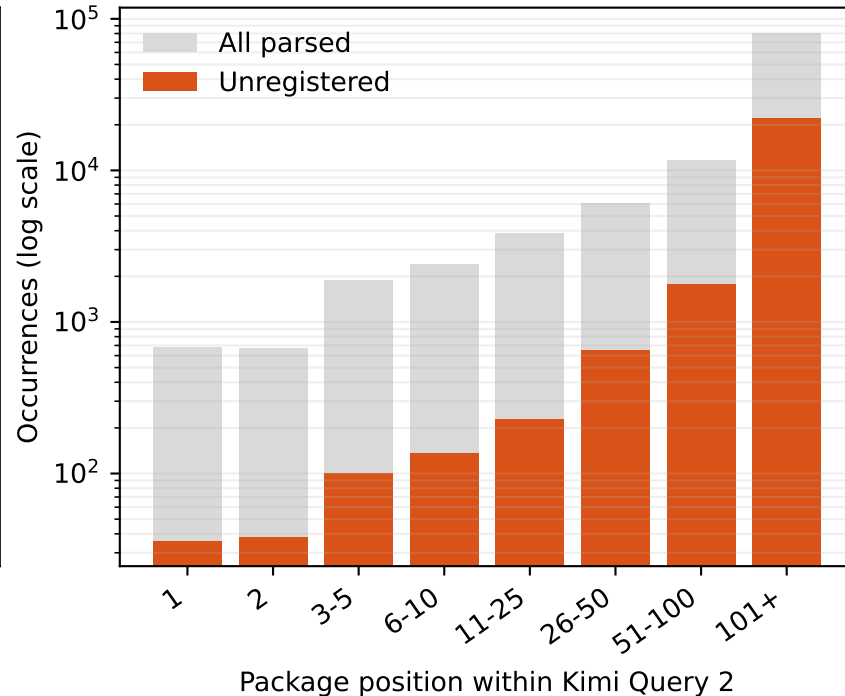
B. Late positions dominate volume
