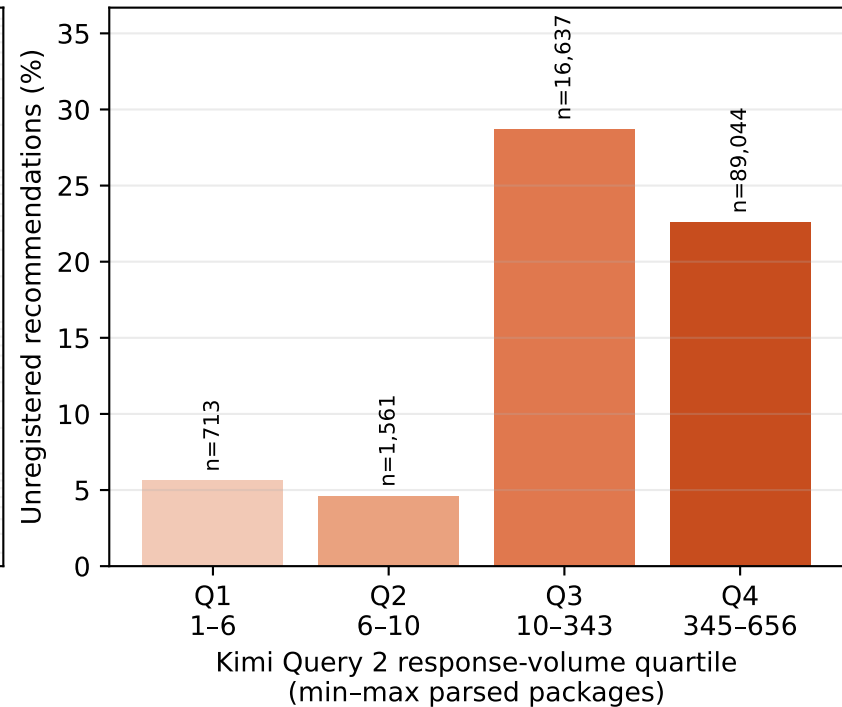
C. Error rate by response volume
