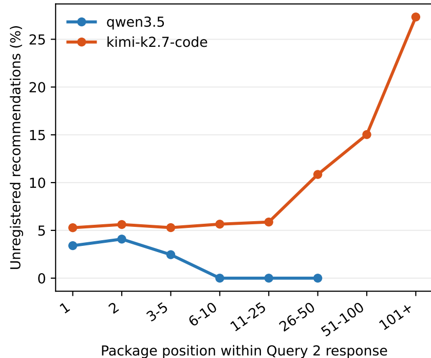
A. Late-list validity collapse
