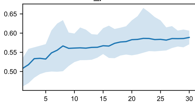
train_time
