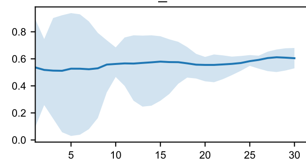
validation_time
