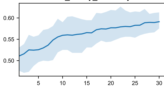
val_precision
