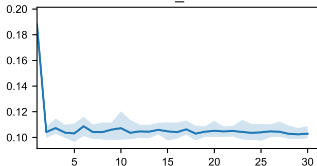
train_pred_time
