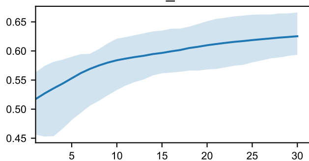
val_recall
