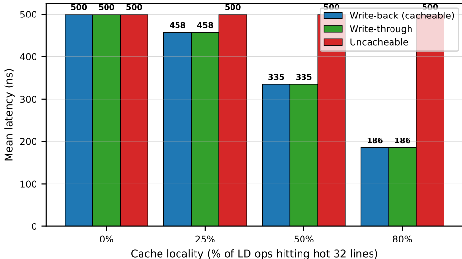
UB §8.3 Load/Store: cache-policy sensitivity (link=100 ns, 64 B)
