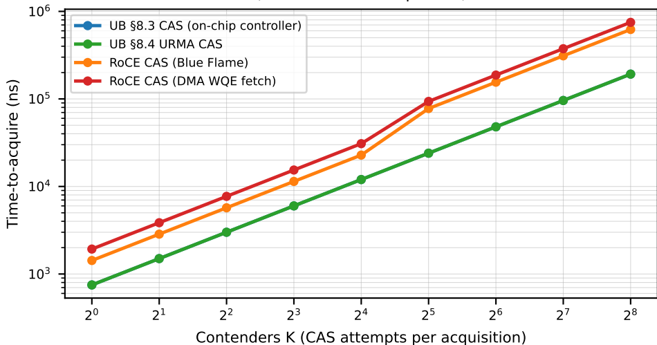
Distributed-lock contention: time-to-acquire vs contenders (link=100 ns, 8 B operand)
